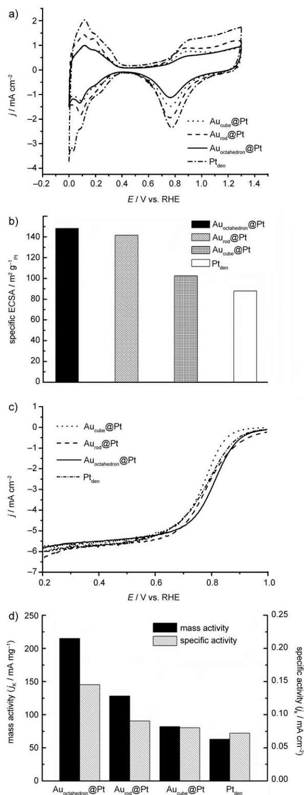
Figure 3. a) CVs of the \text{Au}_{\text{octahedron}}@\text{Pt} , \text{Au}_{\text{rod}}@\text{Pt} , \text{Au}_{\text{cube}}@\text{Pt} , and \text{Pt}_{\text{den}} in 0.1 M \text{HClO}_4 at a scan rate of 50 \text{mVs}^{-1} . The current densities were normalized to the geometric surface area of the GC electrode ( 0.071\text{ cm}^2 ). b) Specific ECSA for each nanostructure. c) Polarization curves for the \text{Au}_{\text{octahedron}}@\text{Pt} , \text{Au}_{\text{rod}}@\text{Pt} , \text{Au}_{\text{cube}}@\text{Pt} , and \text{Pt}_{\text{den}} nanocatalysts in \text{O}_2 -saturated 0.1 M \text{HClO}_4 at a scan rate of 10 \text{mVs}^{-1} and a rotation rate of 1600 rpm. d) Mass- and area-specific activity at 0.8 V versus RHE for the various nanocatalysts.
